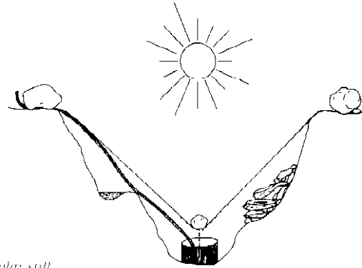
A solar still
