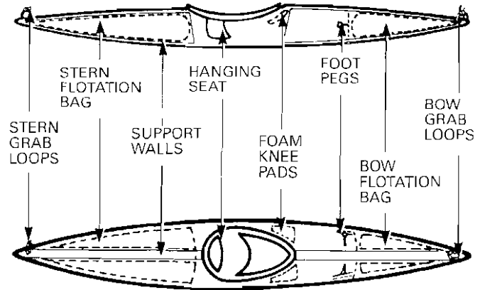
Parts of a Kayak
